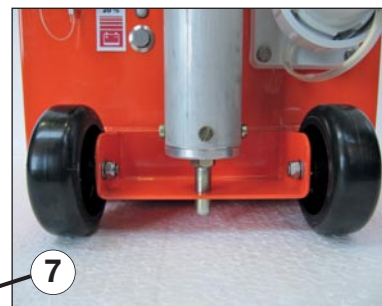
Bottom pin for quick and easy fitting of the mast onto the battery/charger case also equipped with rolling wheels for easy rolling.
